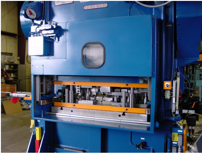
Progressive Tube Sheet Die with Gaggable Sub-dies. The Powered Barrier Guard/ Sound Enclosure in the Open Position.
